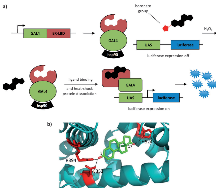
Scheme 1. a) Activation of gene expression by \text{H}_2\text{O}_2 through the oxidation of boronate estrone derivatives. b) X-ray structure of estrone (green) bound to ERα. PDB: 3M1.
